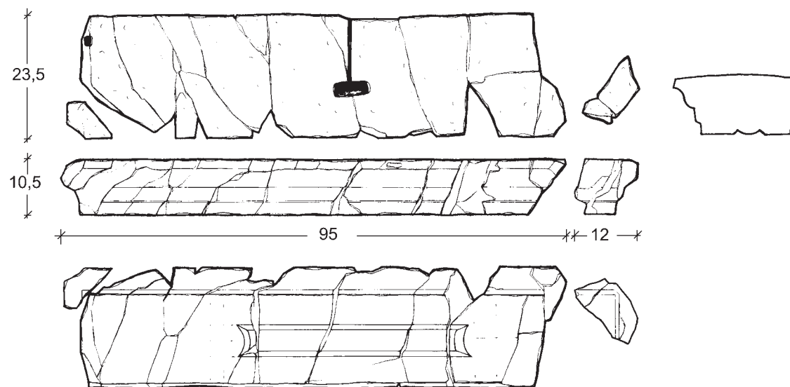
Architrav A 31b-12
